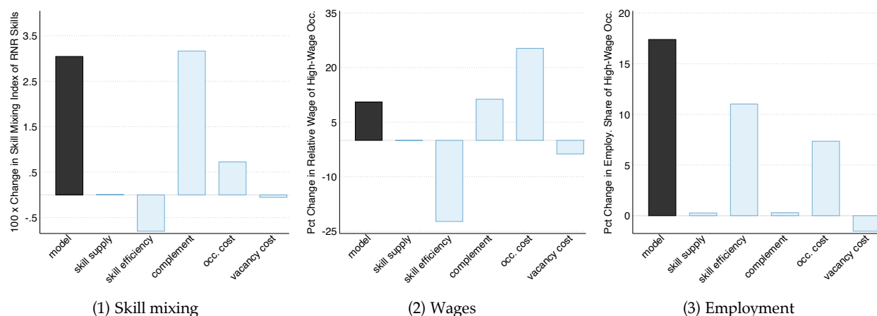
Figure 9: Counterfactual Decomposition
