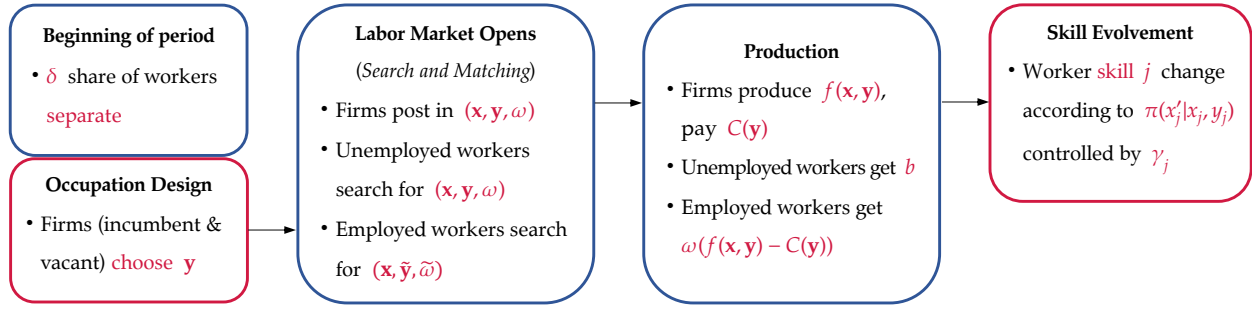
Figure 6: Model Timing
